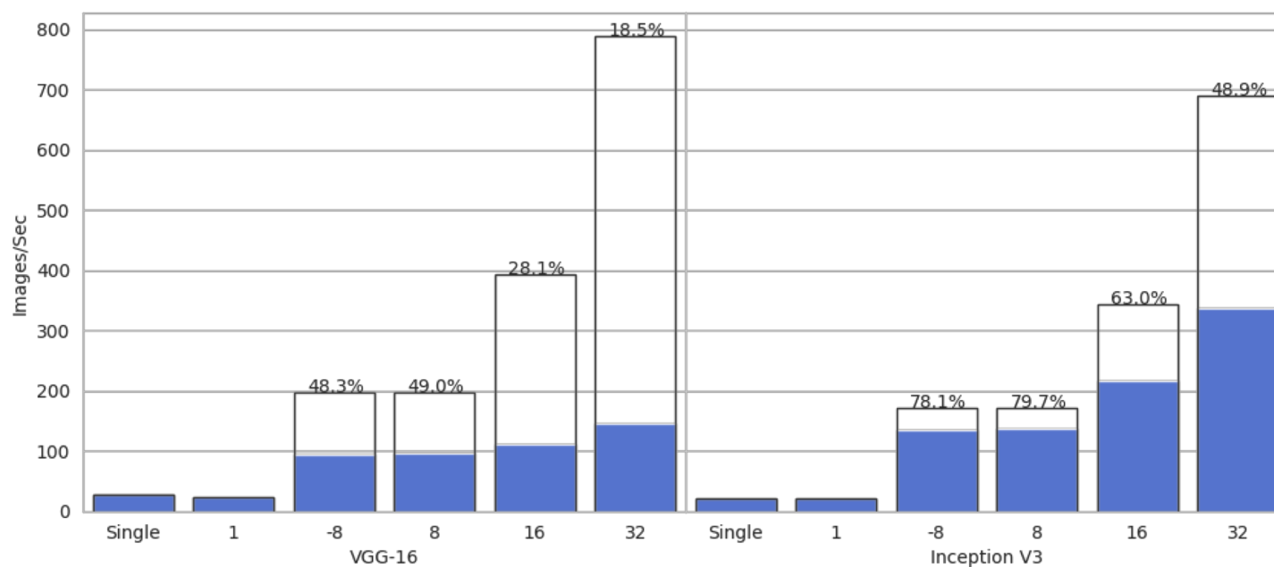
Training with Caltech101 Data on P2.8xlarge Instances
